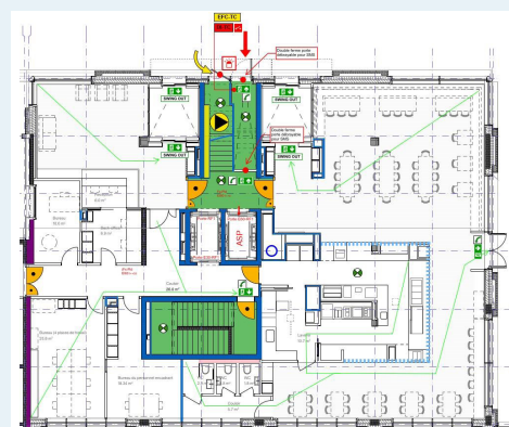
Nos plans - plan de Concept de Protection Incendie
